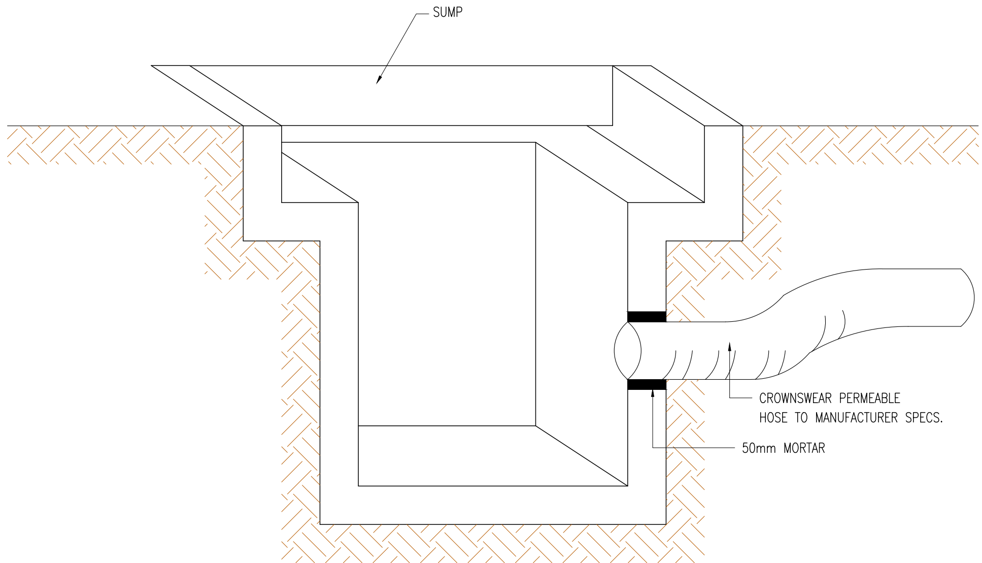
JOINTING TO SUMP
