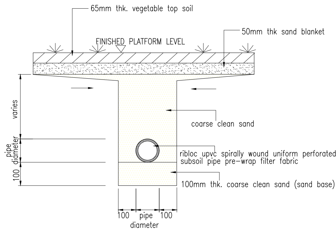
ON-FIELD TRENCH DESIGN
