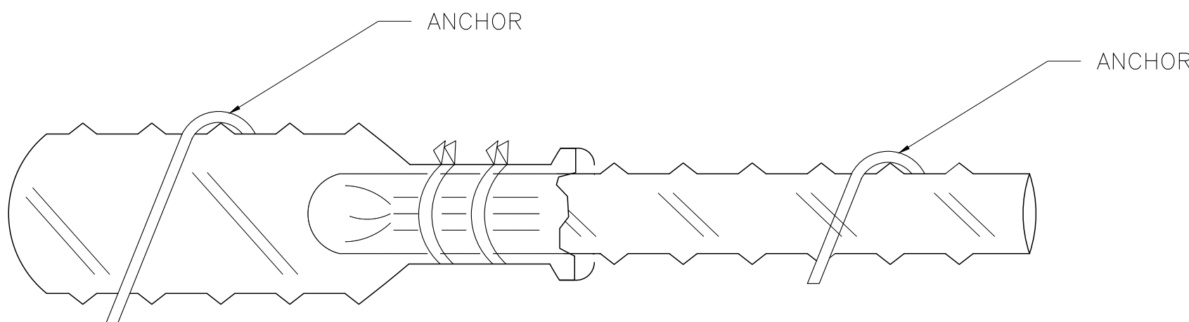
JOINTING DISSIMILAR DIA. HOSES IN STRAIGHT
