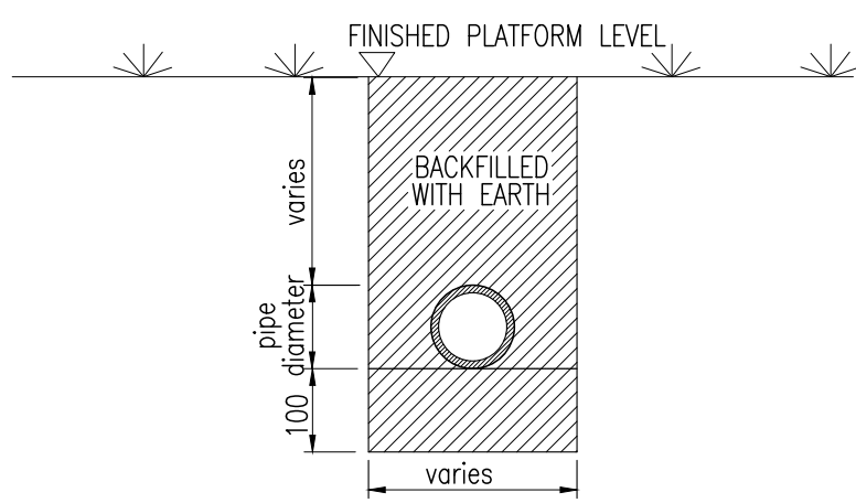
OFF-FIELD TRENCH DESIGN
